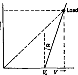
FIG. 7-5.—Voltage-current characteristics of a biased-diode load.
